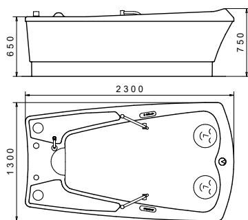
Maße California Twin
