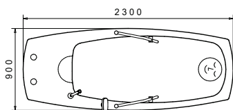
Dimensions Omega cladding
