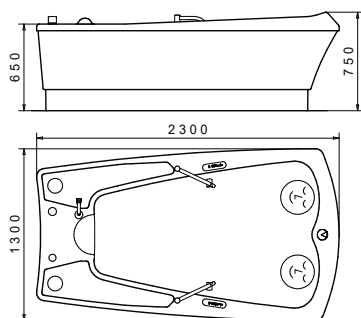
California Twin dimensions
