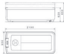
Lady-Spa dimensions standard cladding
