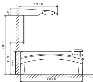
Vichy-Rainbow-Shower Dimensions
