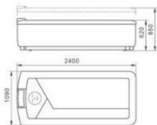
Thermo-Spa dimensions standard cladding
