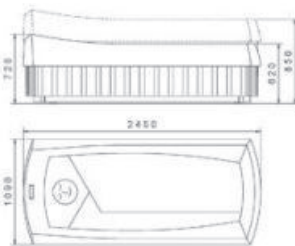
Thermo-Spa dimensions design cladding
