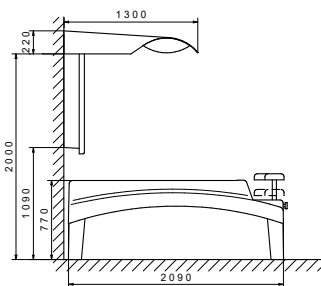
Vichy-Rainbow-Shower Dimensions
